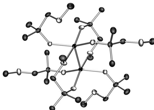
Figure 1. ORTEP view of the structure of complex 2 , ellipsoids at 30% probability, hydrogens are omitted for clarity (tungsten in black, oxygen in white, carbon in grey).
