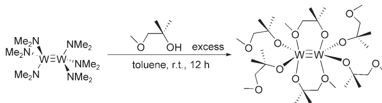
Scheme 2. Reaction scheme for the preparation of the bimetallic complex 2 .
